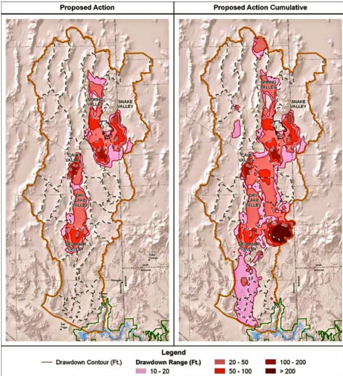
SNWA Proposed Action drawdown and subsidence of full project impacts after 200 years, FEIS page ES-70
